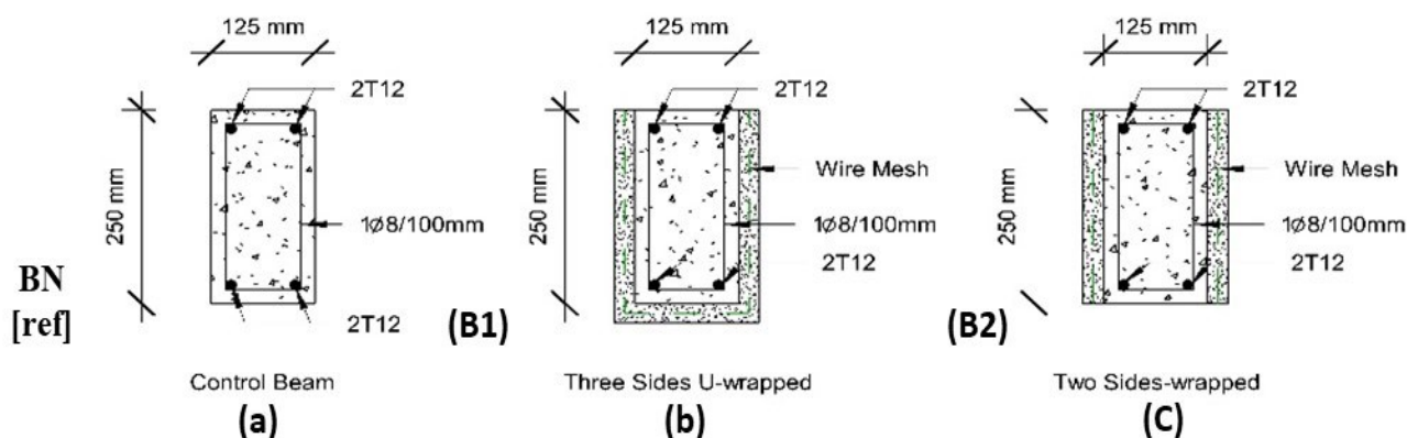
Figure 1. The Cross Sections of Control Beam and Strengthened Beams.
