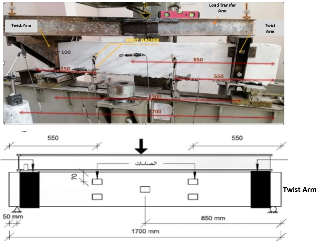
Figure 4. Torsion Test Rig and Sensors Locations.
