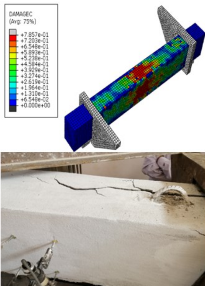
Figure 19. The Cracks Formations of B2 Beam, Experimentally and Analytically.
