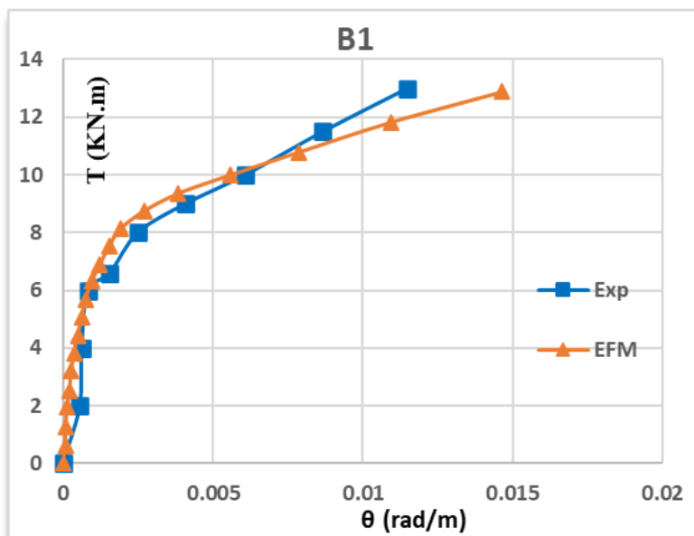
Figure 17. The Torque-Twist Behaviour of B1 Beam, Experimentally and Analytically
