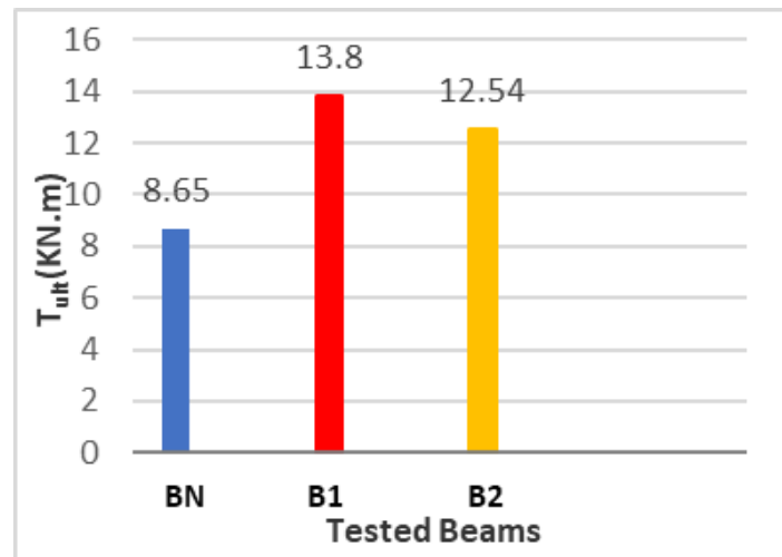
Figure 5. The Average Value of Ultimate Torque of Tested Beams.
