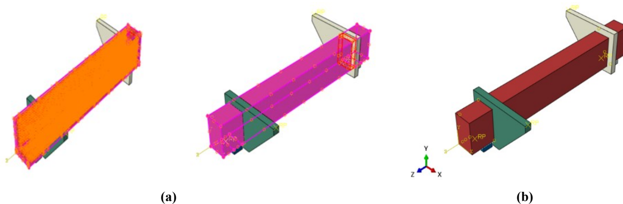
Figure 13. a: The Connection Between the Components of the Model, b: The Final Analytical Model.
