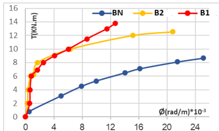
Figure 6. The Relationship Between the Torque and the Twist of Tested Beams.
