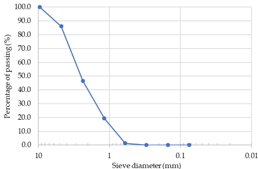
Figure 4. Aggregate Sieve Analysis Results
