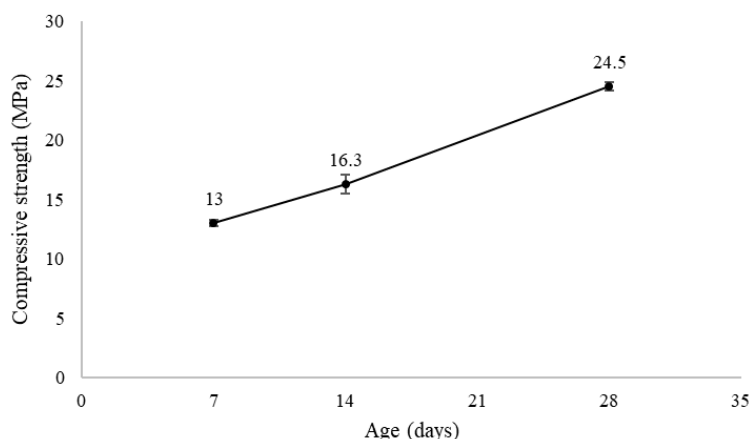
Figure 6. Compressive Strength of the Concrete Mixture.
