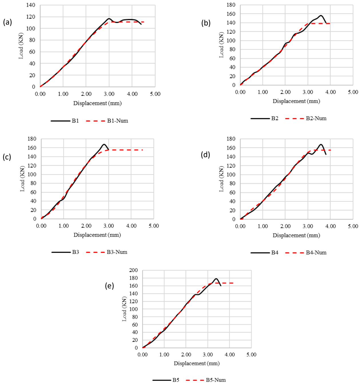
Figure 11. Numerical vs. Experimental Load-Deflection Curves for Beams (a) B1, (b) B2, (c) B3, (d) B4, and (e) B5.
