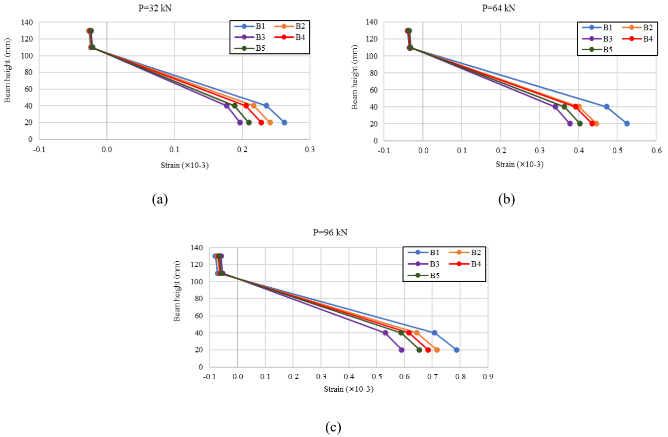
Figure 9. Strain Distribution Plots at (a) 32 kN, (b) 64 kN, (c) 96 kN.
