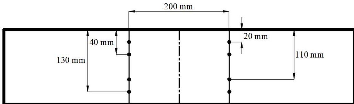
Figure 3. Four Point Bending Test Setup (Dimensions in mm).
