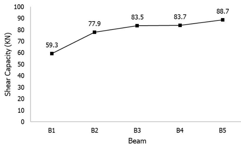
Figure 8. Shear Capacity of Beams B1-B5.
