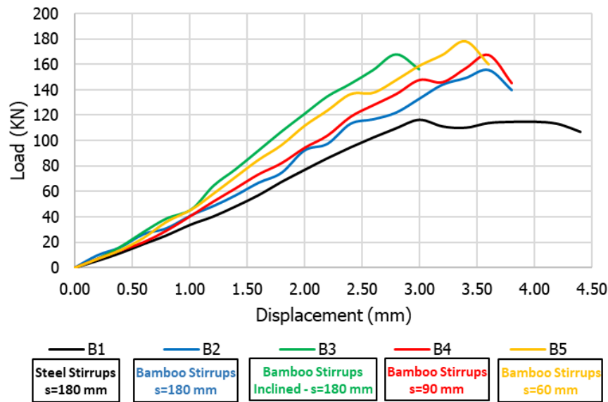
Figure 7. Load-Deflection Curve of Beams B1-B5.
