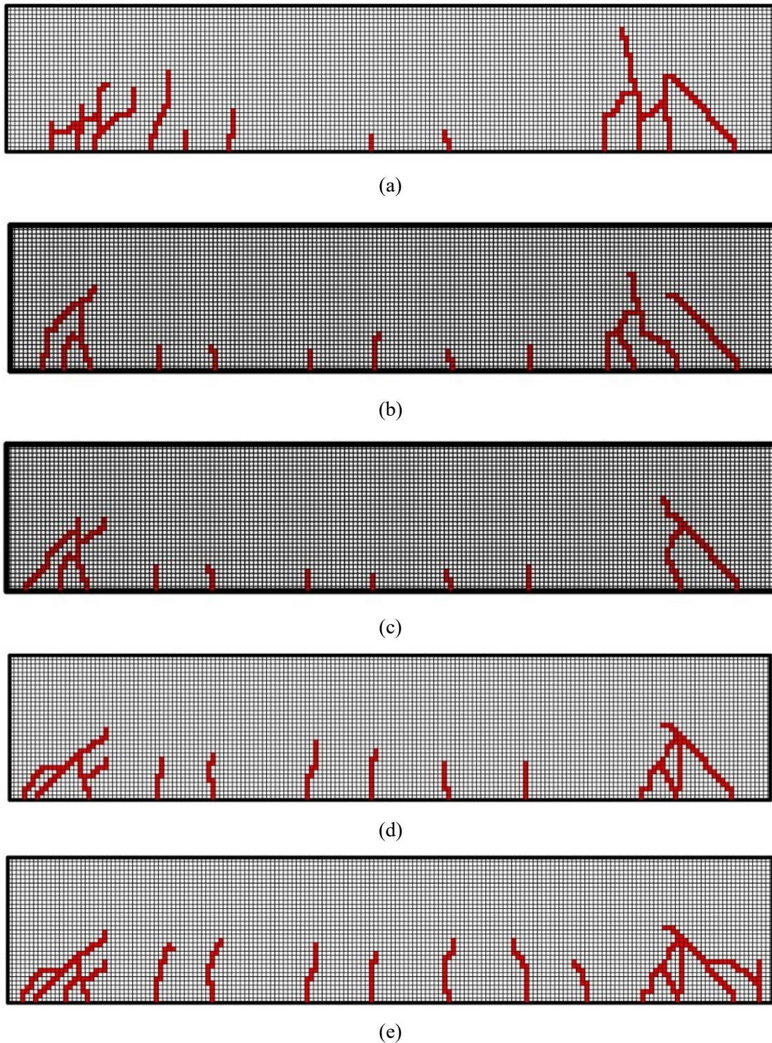
Figure 12. Crack Pattern Generated by Software for Beams (a) B1, (b) B2, (c) B3, (d) B4, and (e) B5.
