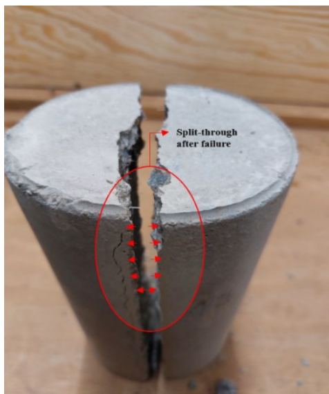
Figure 16. Failure Profile of the GFRC after the Splitting Tensile Strength Test
