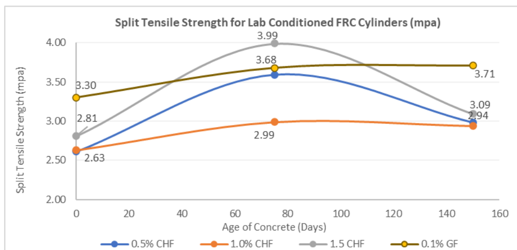
Figure 14. Average Splitting Tensile Strength vs. Age for Lab Conditioned FRC Cylinder Samples
