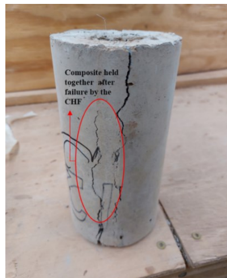
Figure 17. Failure Profile of the CHFRC after the Splitting Tensile Strength Test
