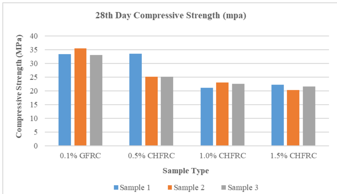
Figure 9. 28 th Day Compressive Strength for the CHFRC and GFRC Cylinder Samples (MPa)
