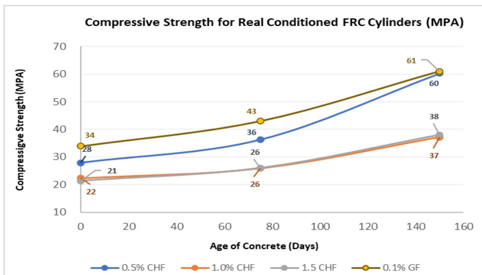
Figure 11. Average Compressive Strength vs. Age for Outside Conditioned CHFRC and GFRC Cylinder Samples.
