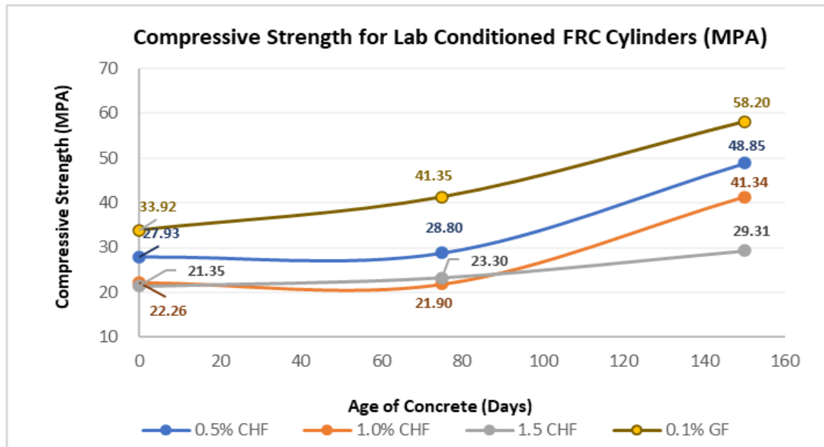
Figure 10. Average Compressive Strength vs. Age for Lab Conditioned CHFRC and GFRC Cylinder Samples
