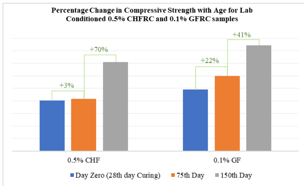
Figure 12. Percentage Change in Compressive Strength with Age for Lab Conditioned 0.5% CHFRC and 0.1% GFRC samples.
