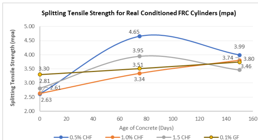
Figure 15. Average Splitting Tensile Strength vs. Age for Outside Conditioned FRC Cylinder Samples
