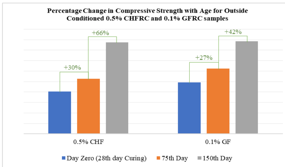
Figure 13. Percentage Change in Compressive Strength with Age for Outside Conditioned 0.5% CHFRC and 0.1% GFRC samples.
