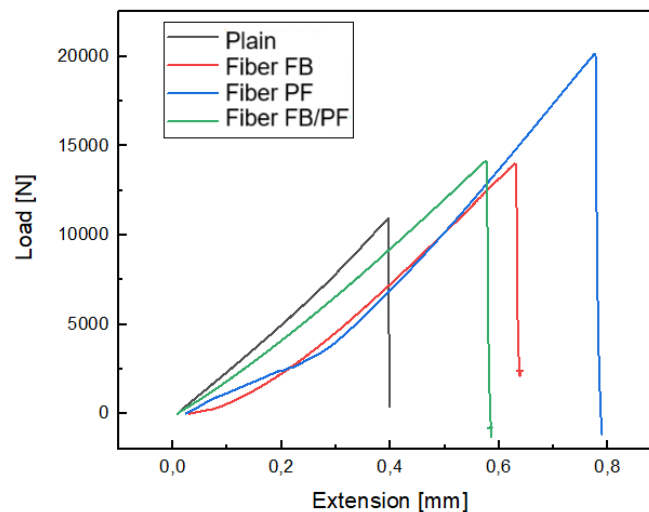
Figure 4. Four-Point Bending Test Results of Combined PF and FB Fibers Compared with Individual Fibers.
