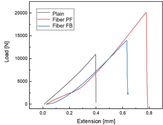
Figure 3. Four-Point Bending Test Results of PF and FB Fibers Compared with the Control Specimen.
