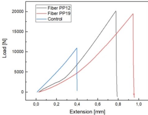
Figure 2. Four-Point Bending Test Results of Polypropylene (PP) Fibers with Varying Lengths Compared to the Control Specimen.
